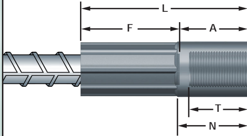
THREADED ROD/BOLTS
